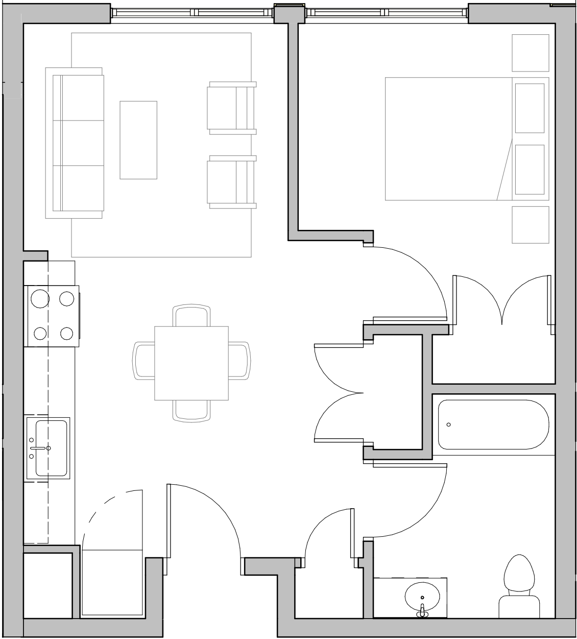
1-Bedroom 545 SF
